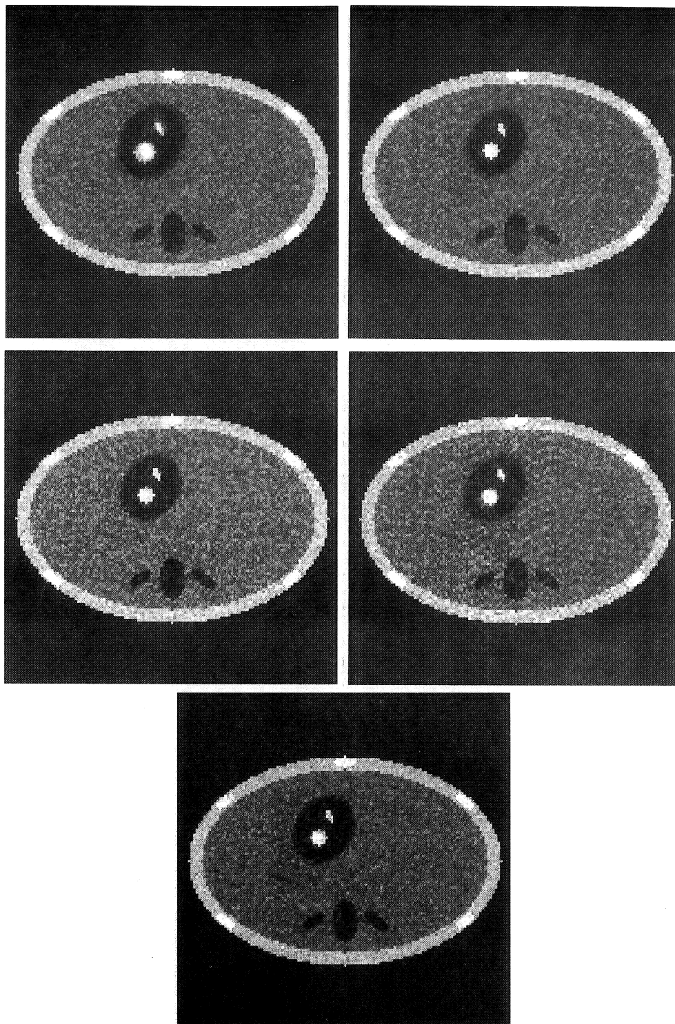
Figure VII.4 . Reconstructions from perturbed data at phase \phi_6 at phase \phi_6 .
